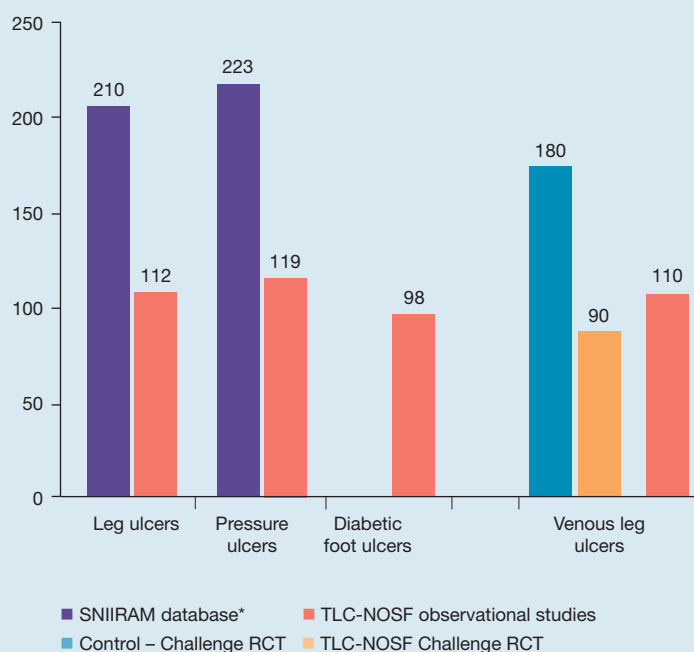
Fig 4. Estimates of time to closure derived from analysed observational studies, SNIIRAM data analysis and from the TLC-NOSF and control dressing groups of the Challenge study
